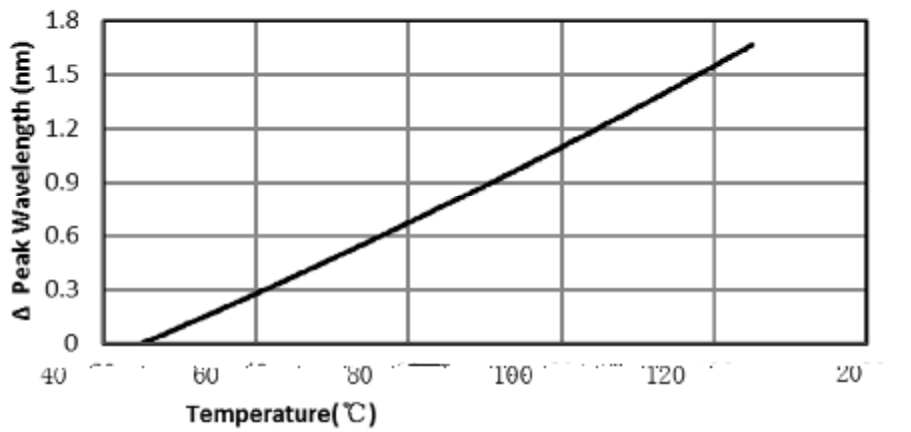
Temperature vs. Peak Wavelength
