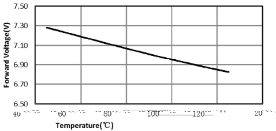
Temperature vs. Forward Voltage
